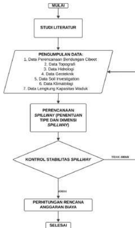
Gambar 3.1. Flowchart Penelitian
